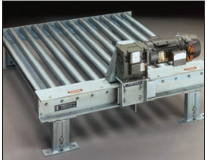
MOTORIZED ROLLER CONVEYOR
